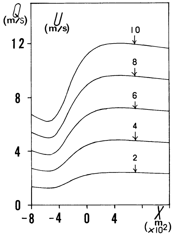
図11 風速III ( Y_0 = 1.500 \times 10^2 \text{ m} , b = 9.000 \times 10^2 \text{ m} )
